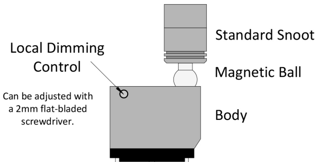
Standard Ionic MX Fitting
