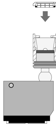
Standard Ionic MX Fitting
