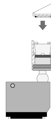
Ionic MX Fitting with Angled Snoot
